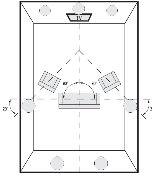
Diagram shows speaker locations for 5.1 and 7.1 systems, when two additional in-ceiling speakers are installed at back of the room.
